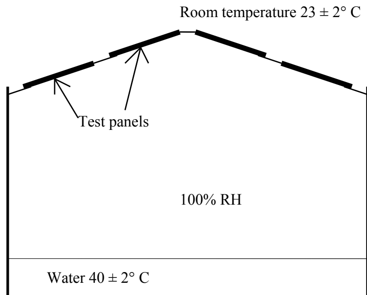
Figure 2 Condensation chamber
